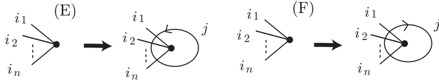
FIGURE 12. (E) passing move L_{s,t}[\sigma_j] for j < s - 1 or L_{s,t}[\sigma_{j-(t+1-s)}] for j > t + 1 , and (F) passing move L_{s,t}[\sigma_j^{-1}] for j < s - 1 or L_{s,t}[\sigma_{j-(t+1-s)}^{-1}] for j > t + 1
