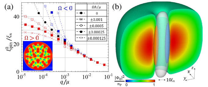
FIG. 3. (a) The q dependence of the width l_{\text{spin}}^{\Omega} of a rotating elliptic vortex with angular velocity \Omega . The single vortex is unstable for larger |\Omega| and smaller q due to the boundary effect. Inset: an elliptic-vortex lattice obtained after the instability due to the boundary effect for \Omega\hbar/\mu = 0.001 and q/\mu = 2^{-11} . (b) The three-dimensional solution of an elliptic vortex in a harmonic trap for \Omega\hbar/\mu = 0.0005 . The isovolume plot shows the region |\Psi_0|^2 c_0/\mu \leq 0.3 for x > 0 with its x = 0 cross-sectional profile. A translucent surface along the z axis represents the isosurface of |\Psi_{\pm 1}|^2 c_0/\mu = 0.15 , to which the two poles of the isosurfaces s_y c_0/\mu = \pm 0.7 are attached (red for positive and blue for negative).
