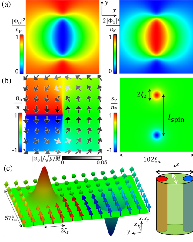
FIG. 1. The cross-sectional profile of an elliptic vortex for q/\mu = 2^{-17} \approx 7.6 \times 10^{-6} . (a) The left and right sides show the profiles of |\Phi_0|^2/n_p and 2|\Phi_1|^2/(2n_p) , respectively. The density |\Phi_{-1}|^2 (not shown) is the same as |\Phi_1|^2 . (b) The vector field on the left shows \mathbf{v}_0 = (\hbar/M)\nabla\Theta_0 , with the background plot of \Theta_0 = \arg \Phi_0 . The phase \arg \Phi_{\pm 1} is homogeneous inside the core (not shown). The spin density s_y is plotted on the right, while s_x = s_z = 0 . (c) Left: the texture of the unit vector \mathbf{g}/|\mathbf{g}| (arrow) in Eq. (3). The color of the arrows and the surface correspond to \Theta_0 and s_y in (b), respectively. Right: schematic of the three-dimensional structure of the vortex core. The distance l_{\text{spin}} between the two spin spots with opposite transverse magnetization (blue and red) is determined by the balance between the hydrodynamic potential and the elastic potential by the AF soliton (green). The width ( \sim l_{\text{spin}} ) and thickness of the core are represented by black and white arrows, respectively.
