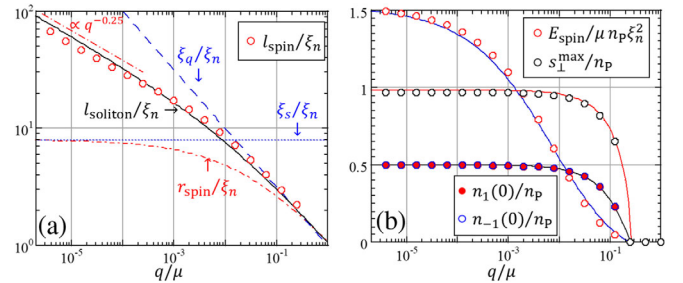
FIG. 2. (a) The q dependence of l_{\text{spin}} . The solid curve represents the evaluation by Eq. (12). All lengths are rescaled by \xi_n . (b) The q dependence of the spin interaction E_{\text{spin}} , the maximum spin density s_{\perp}^{\text{max}} = \max(s_y) , and the core density n_{\pm 1}(0) . The solid curve tracing the data corresponds to an analytic formula (see text).
