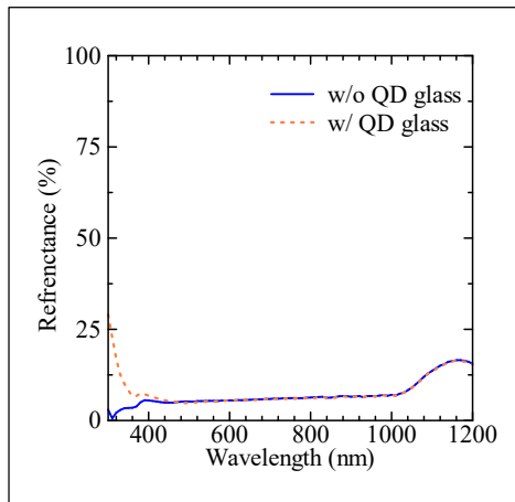
Figure S5. Surface reflectance of Si solar cells with and without the QD glass.
