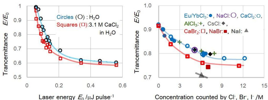
Fig. 3. Left: The transmittance of fs laser pulses for \text{H}_2\text{O} ( \circ ) and 3.1 M \text{CaCl}_2 aqueous ( \square ) (6.2 M as \text{Cl}^- ) solutions. The laser pulse was 80 fs negative chirp and focused into the center of a 1 cm long cell through a 12 cm focus lens. Right: Transmittances of the same fs pulses with 0.09 \mu\text{J} pulse energy for various salt solutions. The solid lines represent guides. The upper points on the blue guideline are for chloride metal salts.
