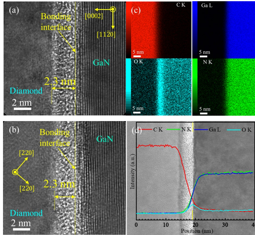
Figure 5. HRTEM images taken along (a) GaN [1\bar{1}00] zone axis and (b) diamond [001] zone axis of a 700 °C-annealed GaN/diamond heterointerface. (c) EDS mappings of the heterointerface. (d) X-ray intensity profiles for C, Ga, O, and N atoms (red, blue, cyan, and green, respectively) across the heterointerface. The inset TEM image back in (d) indicates the corresponding location of the measured X-ray intensity profiles for C, N, Ga, and O atoms.
