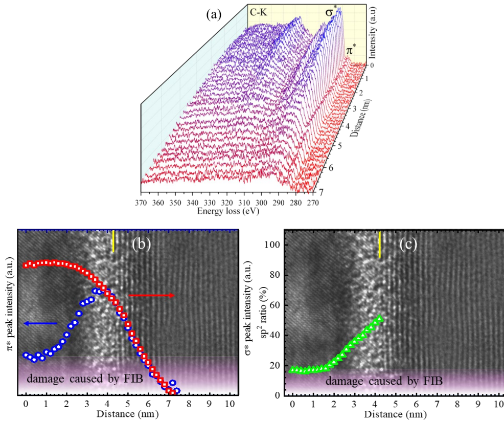
Figure 9. (a) C-K edge EELS spectra obtained from line scan across a 1000 °C-annealed GaN/diamond heterointerface. (b) \pi^* and \sigma^* peak intensities. (c) sp^2 ratio deduced from EELS spectra as a function of the scanned distance. The inset back in (b) and (c) shows TEM images of a 1000 °C-annealed GaN/diamond heterointerface. The area filled with lavender in (b) shows the averaged \pi^* peak intensity of EELS spectra caused by FIB.
