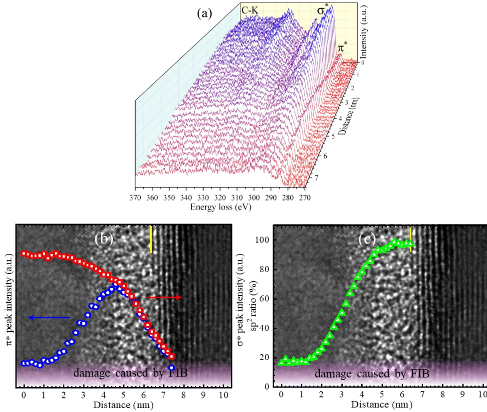
Figure 8. (a) C - K edge EELS spectra obtained from line scan across a 700 °C-annealed GaN/diamond heterointerface. (b) \pi^* and \sigma^* peak intensities and (c) sp^2 ratio deduced from EELS spectra as a function of the scanned distance. The inset back in (b) and (c) shows TEM images of a 700 °C-annealed GaN/diamond heterointerface. The area filled with lavender in (b) shows the averaged \pi^* peak intensity of EELS spectra caused by FIB.
