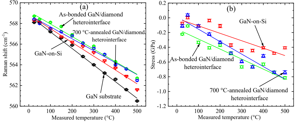
Figure 2. (a) Raman shift of GaN in a stress-free GaN substrate, GaN layer grown on Si substrate, the as-bonded and 700 °C-annealed GaN/diamond heterointerfaces and (b) biaxial stress in the GaN layers grown on Si, the as-bonded and 700 °C-annealed GaN/diamond heterointerfaces as a function of measured temperature. Negative sign indicates a compressive stress. The phonon frequency shift contributing to measured temperature was subtracted after comparison with a calibration performed on a stress-free GaN substrate.
