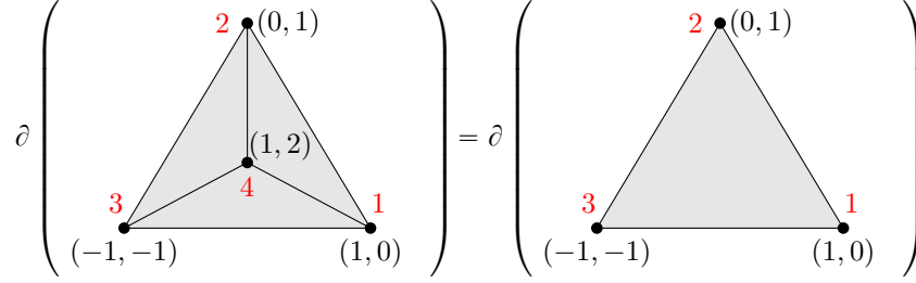
FIGURE 3. Two simplicial chains with vector functions having the same boundary
