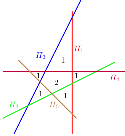
FIGURE 2. Duistermaat–Heckman function of the multi-polytope P .
