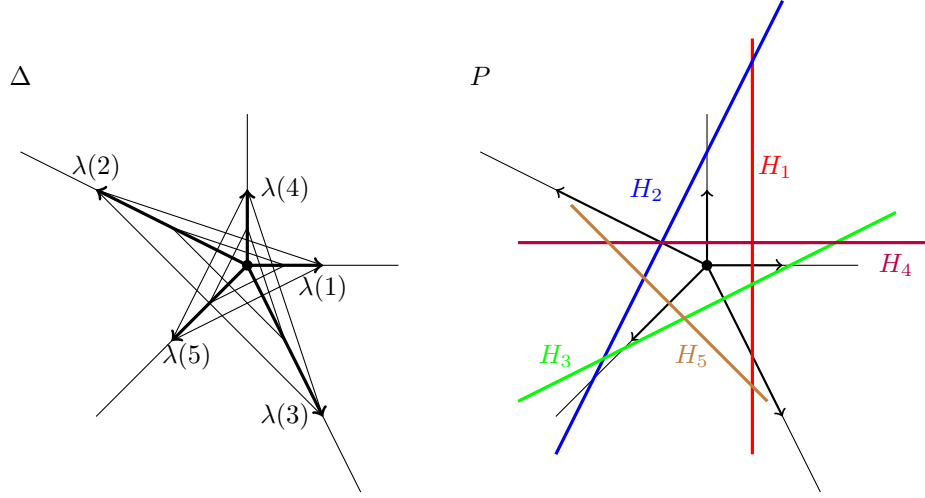
FIGURE 1. Example of a multi-fan \Delta and a multi-polytope P based on it.
