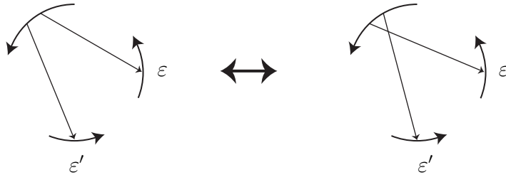
FIGURE 7. The move of Gauss diagrams corresponding to the forbidden move \Phi_t , where \epsilon, \epsilon' = + or - .
