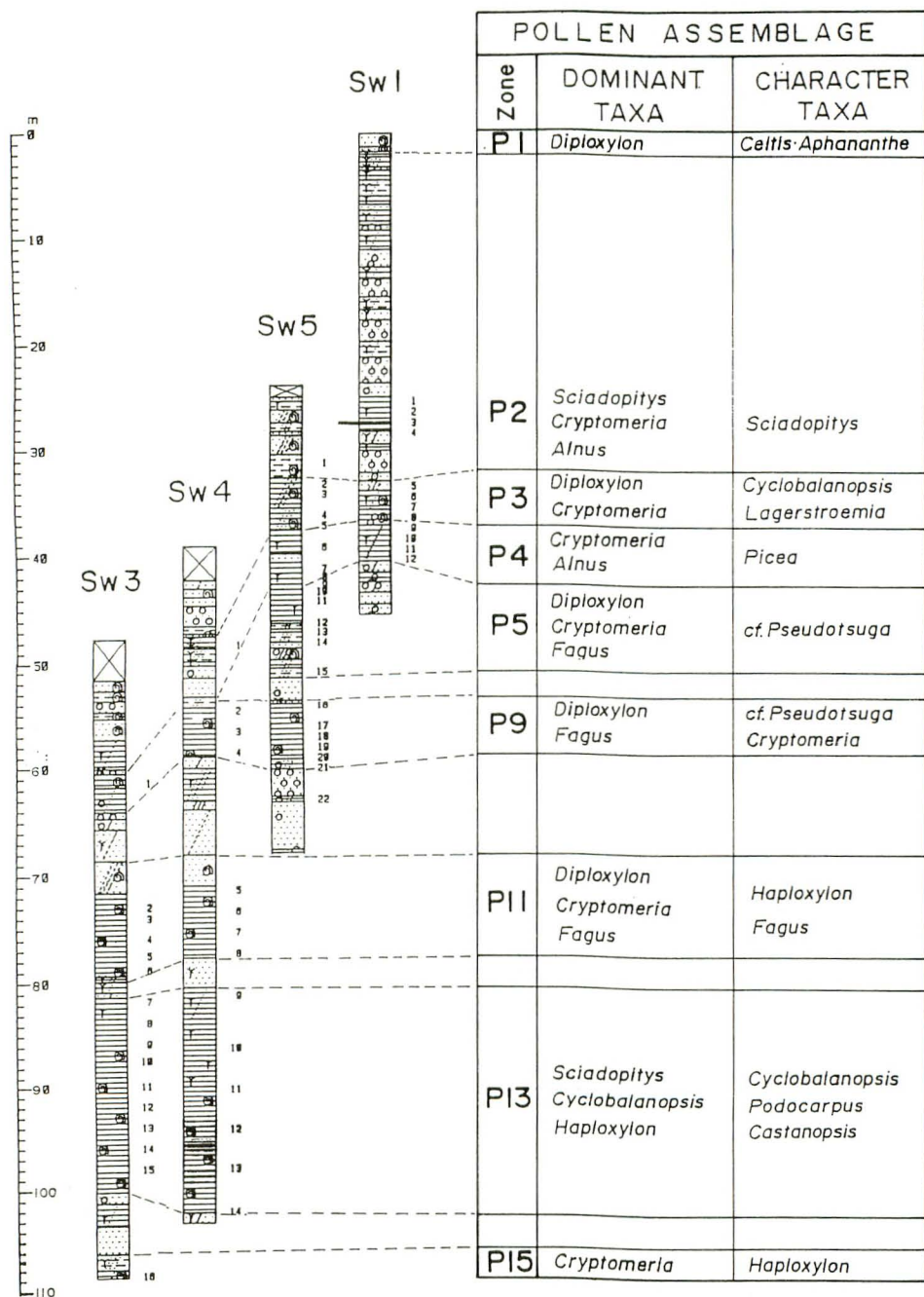
Fig. 5. Lithologic and pollen successions in onshore of Senuu.
