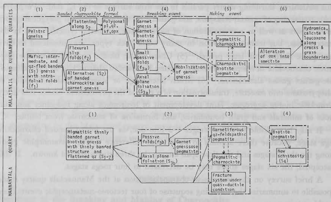
Fig. 32. Summary and comparison of structural and metamorphic events between the Malayinkil and Kunnanpara quarries and the Mannantala quarry.
