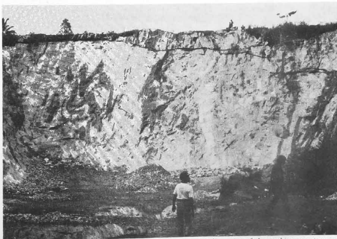
Fig. 3. Paleozomic folded ( f_2 , modified by later f_3 tectonics) alternation of charnockite-garnet gneiss (north wall of the Kunnanpara quarry). In this outcrop, the mobilization of the garnet gneiss is dominant (cf Fig. 12).
