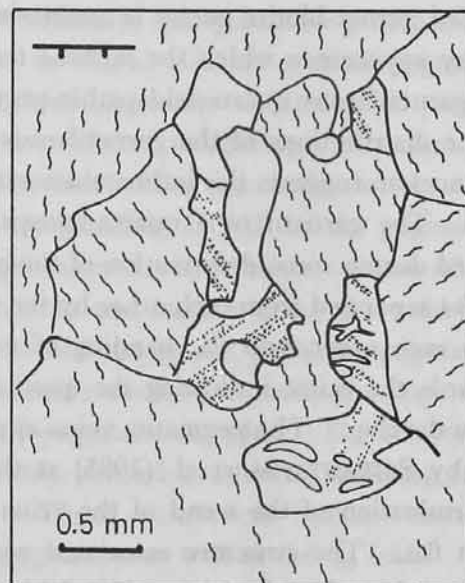
Fig. 28. Microstructure of salic minerals, specimen 86010301B.
