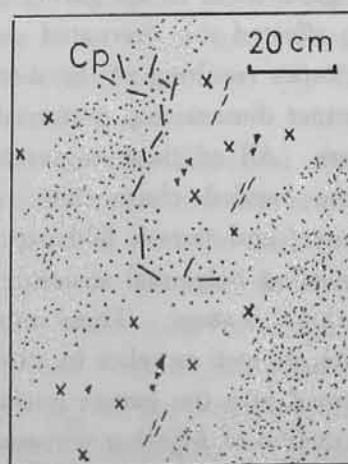
Fig. 31. Pegmatitic charnockite developed over the garnet gneiss (northern part of the eastern cliff of the Malayinkil quarry).
