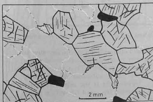
Fig. 19. General microstructure of the basic charnockite, specimen 86011101A.
