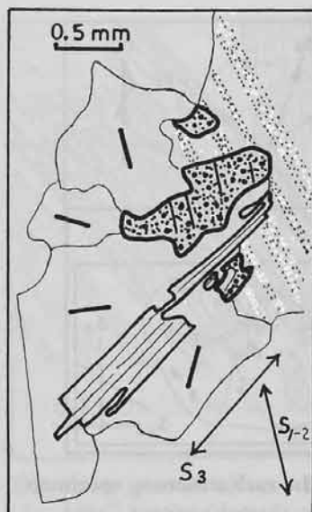
Fig. 26. Occurrence of orthopyroxene and biotite, specimen 86010301A.
