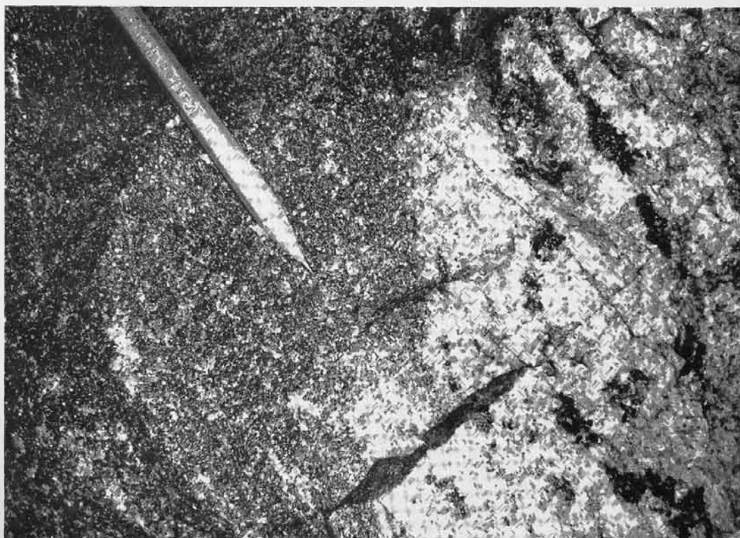
Fig. 11. Retrogression of the charnockite (very dark, left-most part) into the garnet gneiss (light, right half) through the garnet-biotite gneiss (dark, around the top of the pencil) (lower left part of Fig. 10; the figure orientation is rotated).
